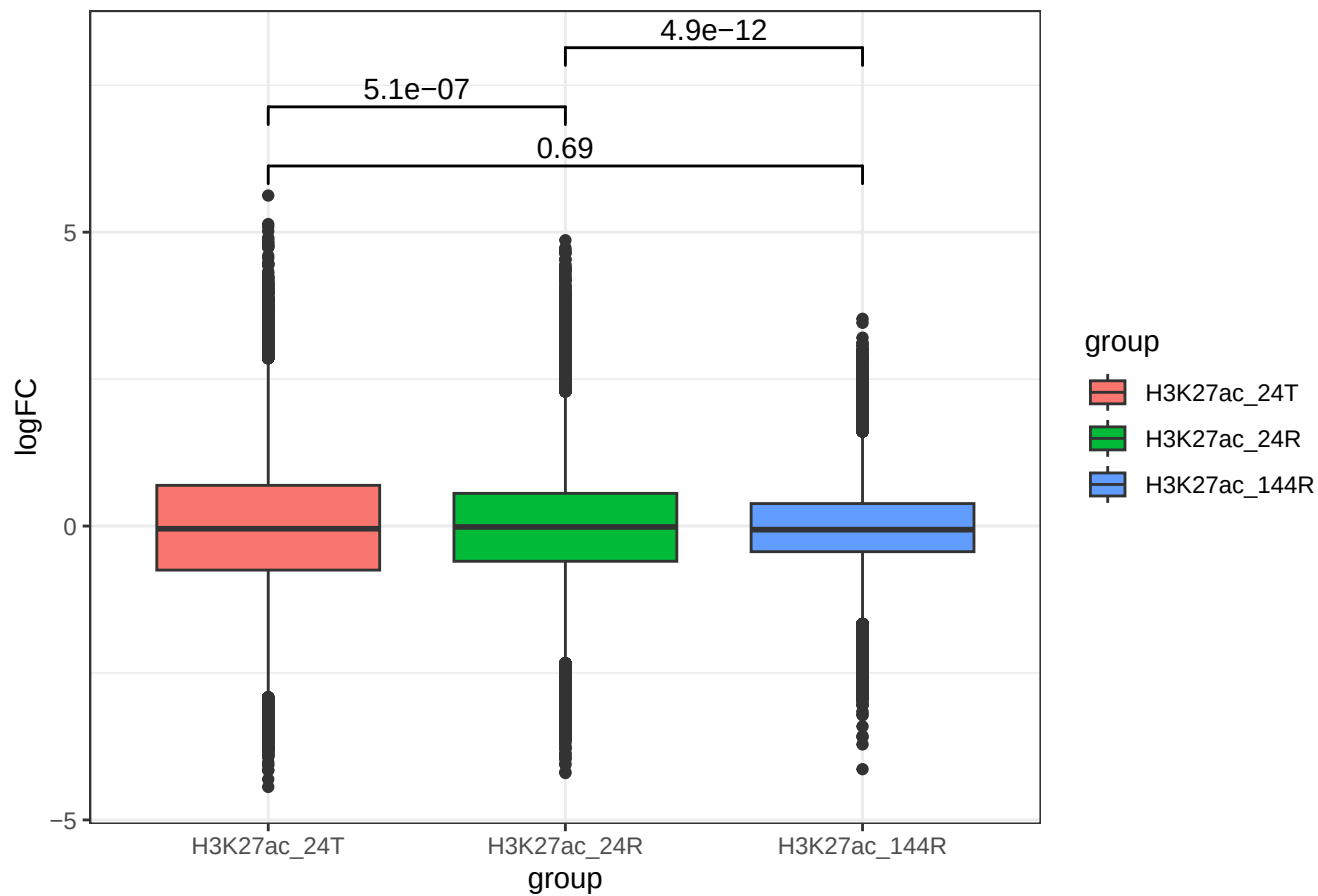
LFC across time for H3K27ac
